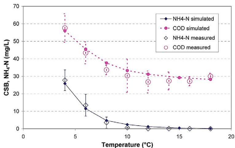
FIG. 8. Measured and simulated chemical oxygen demand (COD) and NH 4 -N effluent concentrations using the modified parameter set (Langergraber, 2007).
