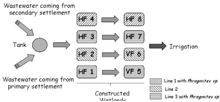
FIG. 13. Schematic sketch of pilot plant in San Michele di Ganzaria (Toscana et al., 2006).
