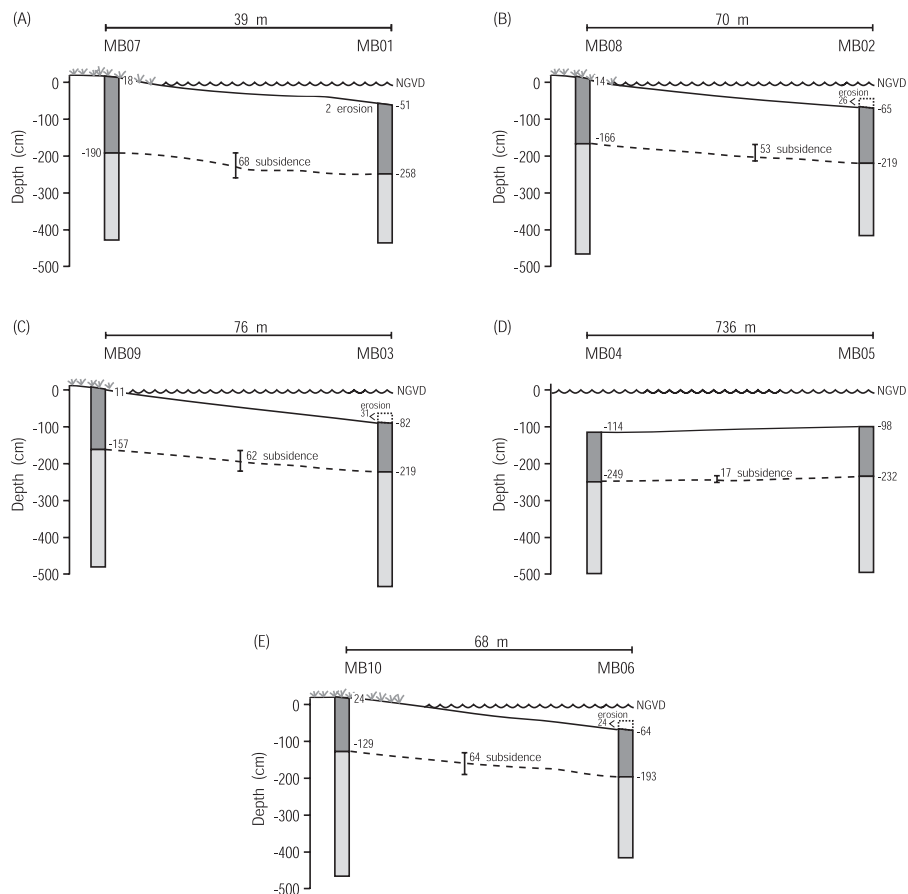
Figure 4. Stratigraphic correlations for marsh and open-water core pairs illustrate the magnitude of subsidence and wetland erosion (in centimeters) at the Madison Bay wetland loss hot spot. The upper stratigraphic unit represents the peat and organic mud facies, whereas the lower unit includes the three other facies. Locations shown in Figure 2.
