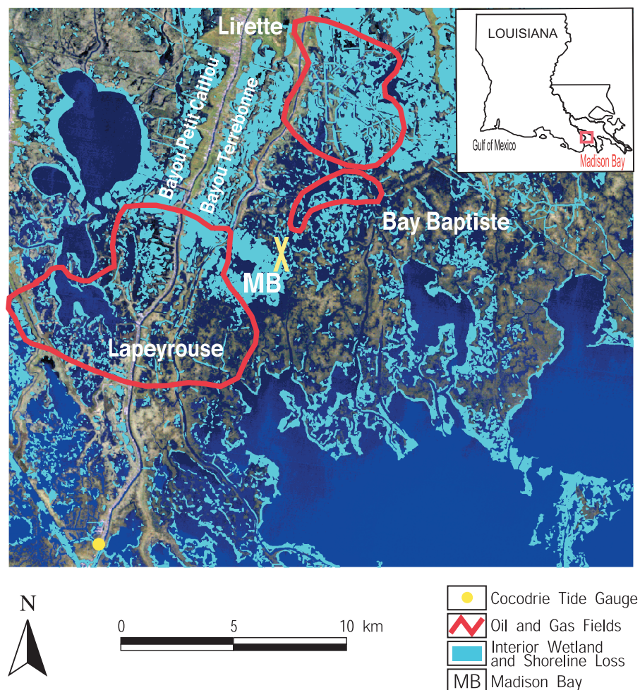
Figure 1. Map of south-central Louisiana showing the location of Madison Bay (MB), the Cocodrie tide gauge, and the distribution of wetland losses relative to producing oil and gas fields. Wetland loss (1930–1990) from Britsch and Dunbar (1996). General geographic position of the yellow X is lat. N29°21'50", long. W90°34'45".
