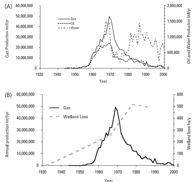
Figure 5. Temporal comparison of (A) annual volumes of fluid produced from the Lapeyrouse field (data from the Louisiana Department of Natural Resources) and (B) wetland losses in the Dulac quadrangle (data from Britsch and Dunbar, 1993).
