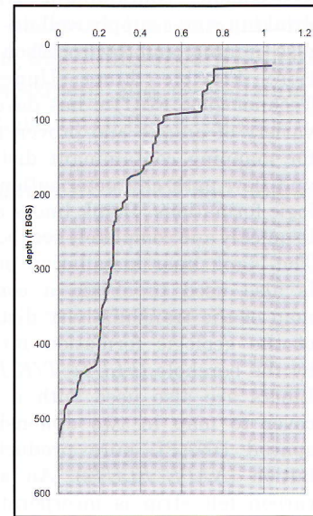
Figure 2. Velocity profile in borehole.
