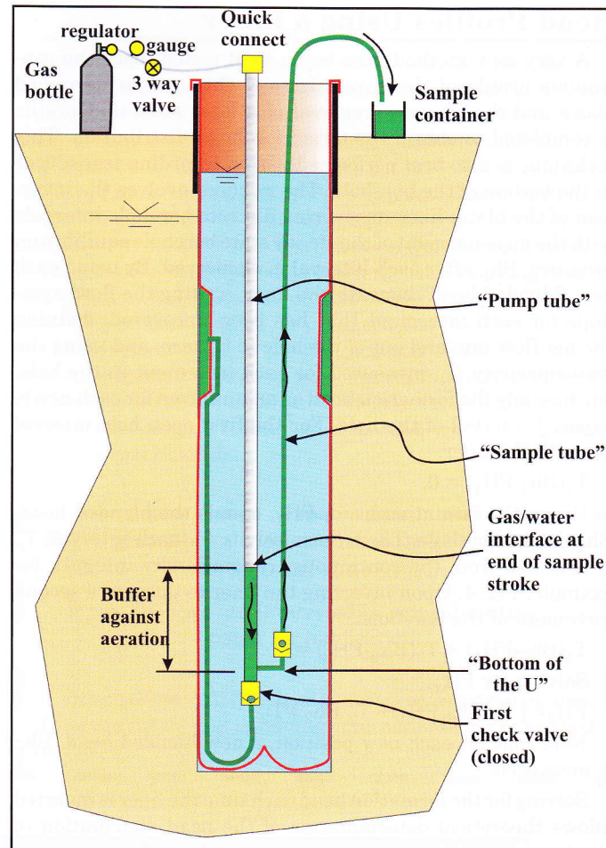
Figure 9. Pumping Procedure.
