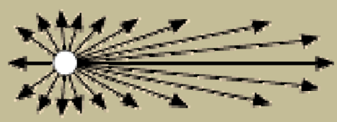
Mie Scattering, larger particles
