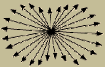
Rayleigh Scattering
