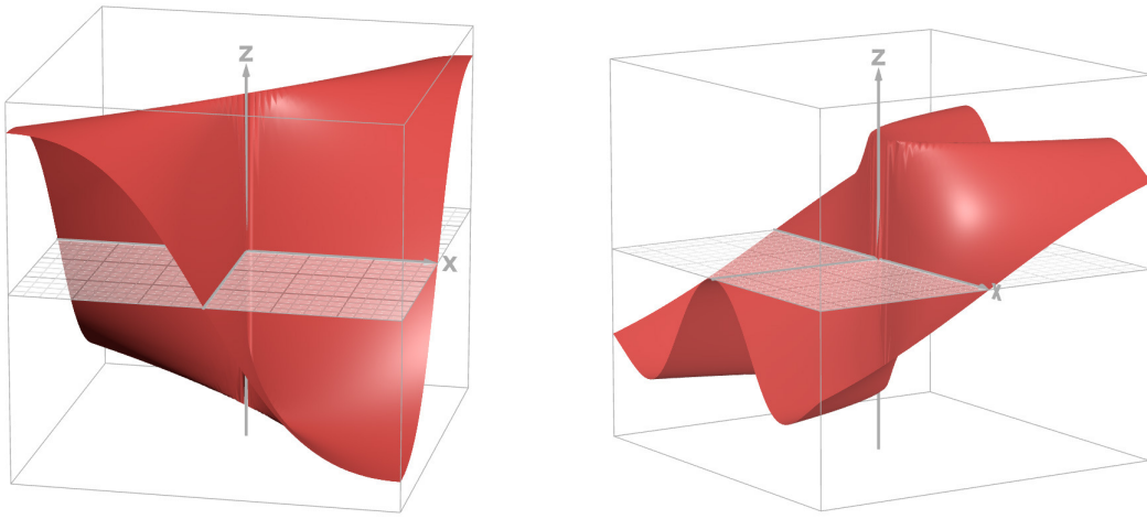
FIGURE 1. z = \frac{xy}{x^2 + y^2} .
